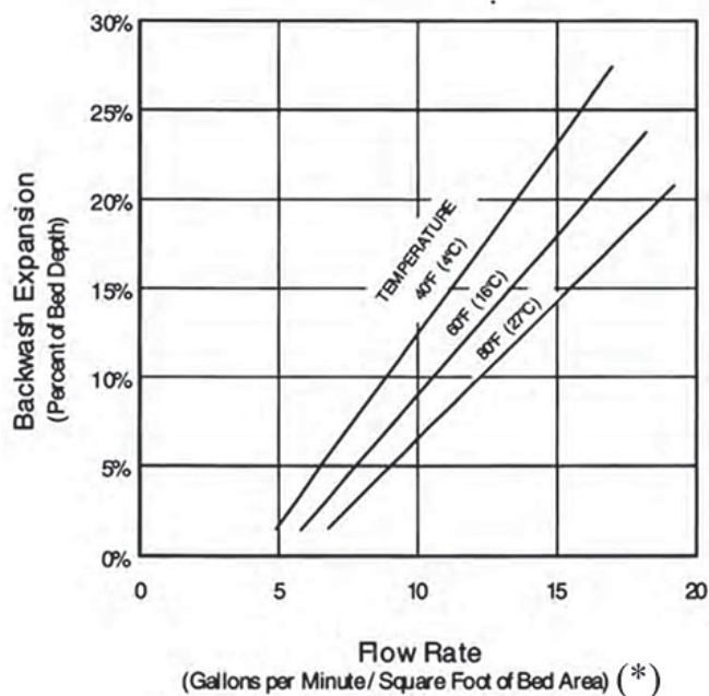
BACKWASH BED EXPANSION
