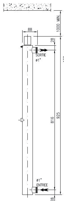
UV412
